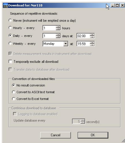
NorMonitData management menu
